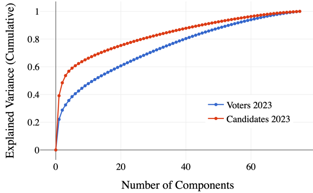
Figure 11: PCA explained variance for voter and candidate answer profiles in the 2023 dataset. The plot shows the cumulative explained variance as a function of the number of principal components for both voters and candidates.
